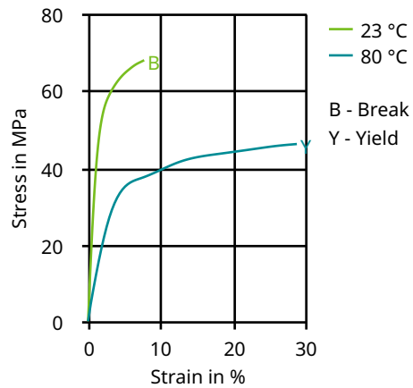
Stress-strain (cond.)
