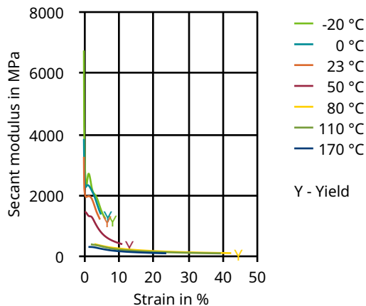
Secant modulus-strain (dry)
